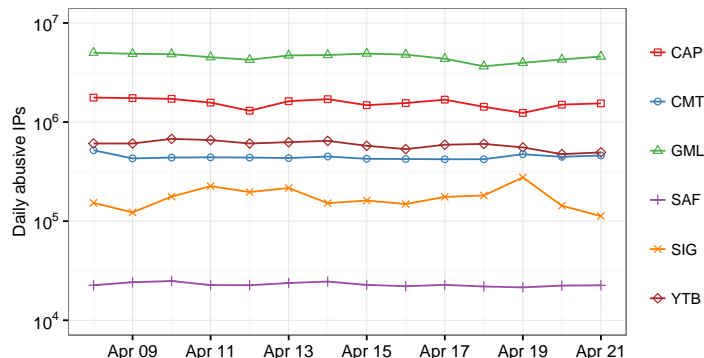
Fig. 1: Daily volume of IP addresses reported by various Google services for abuse. We observe an order of magnitude more spam bots than all other threats.
